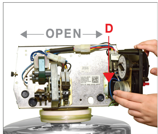
Figure 11 - Premier 2250SE timer
