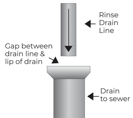
Figure 5 - Air Gap Illustration
