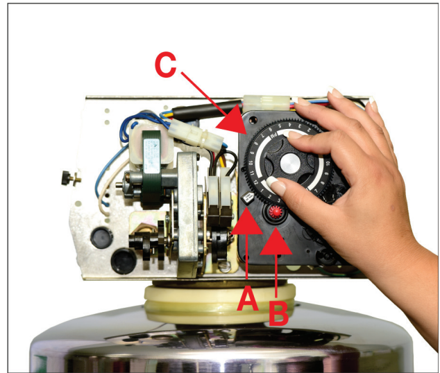
Figure 12 - Premier 2250SE timer
